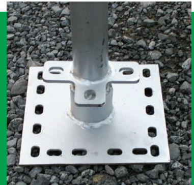
Stainless Steel Foot Plate Schick Enterprises makes 1 to 4-way posts
